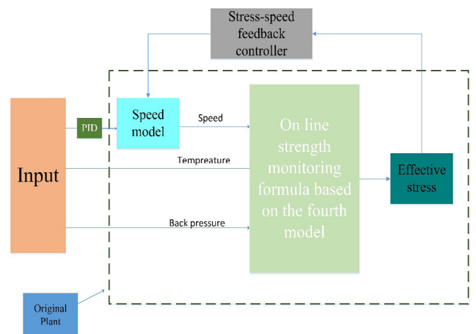
Figure 17: Structure diagram of stress-speed feedback control model.
