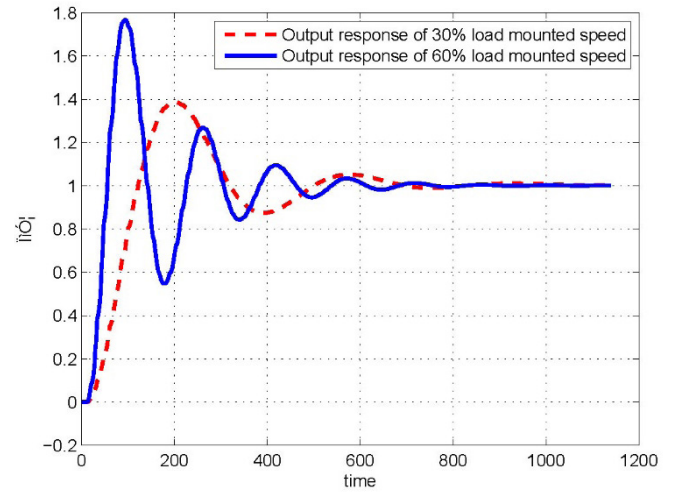
Figure 16: Speed response of 30% and 60% load respectively.
