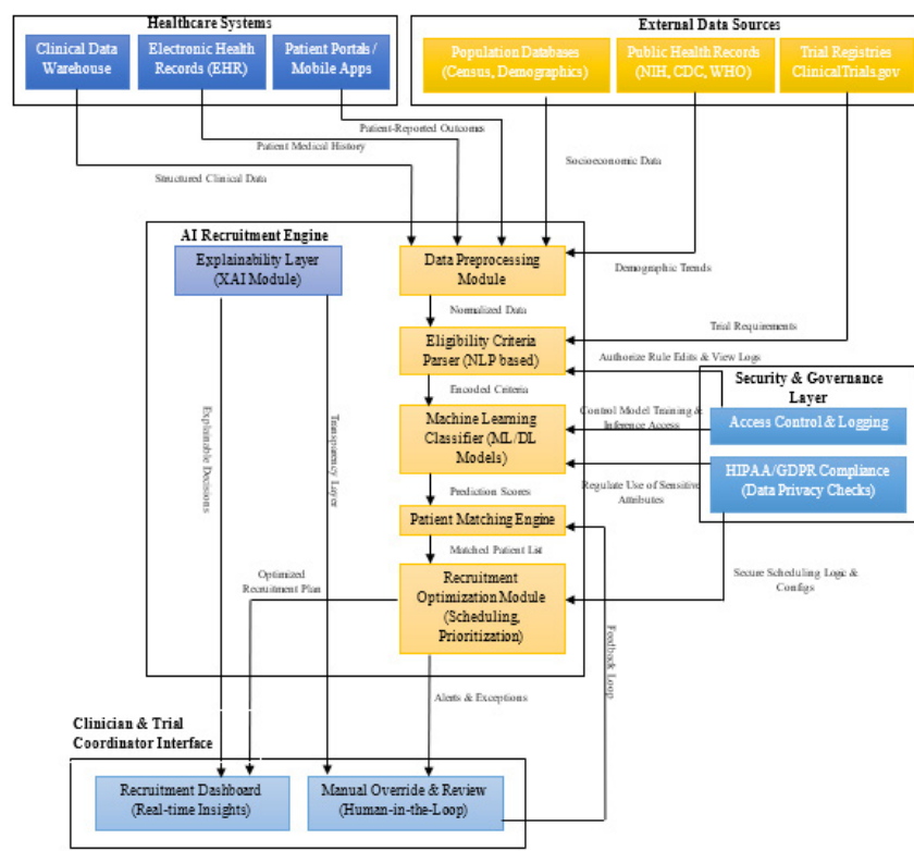
Figure 1: AI-Driven Patient Recruitment Architecture.
