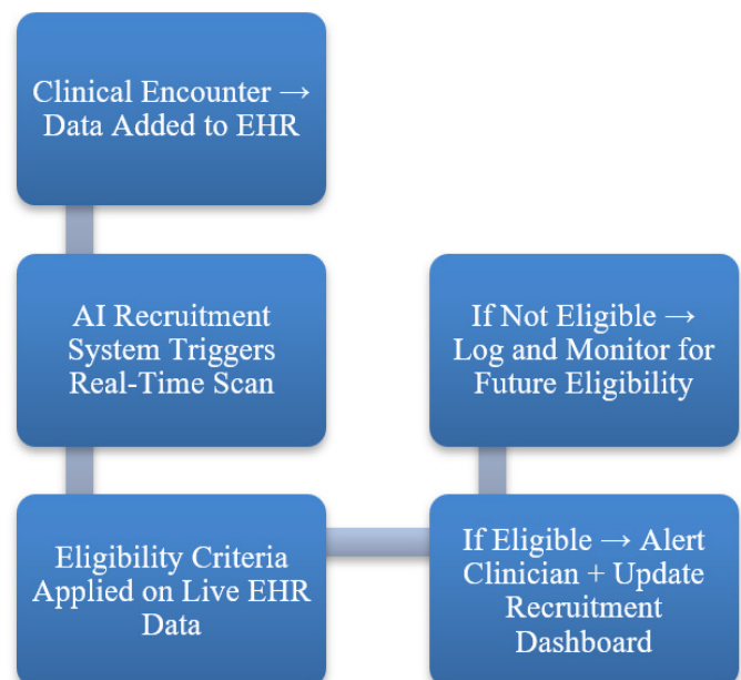
Figure 2: Real-Time Integration with EHR Systems.
